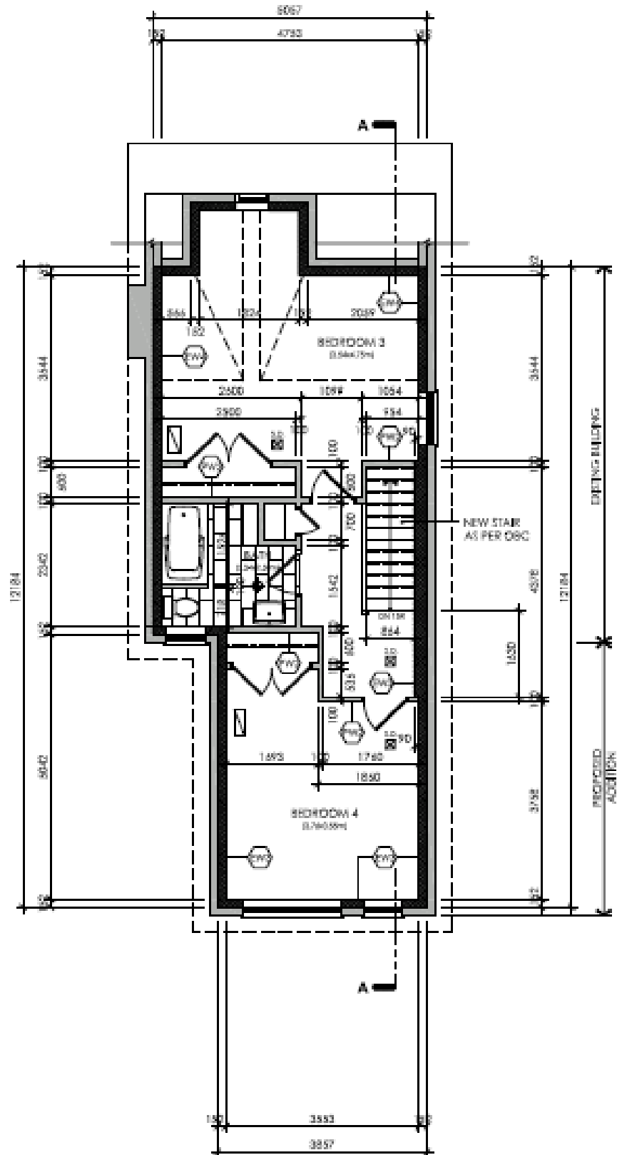
3 rd Floor
