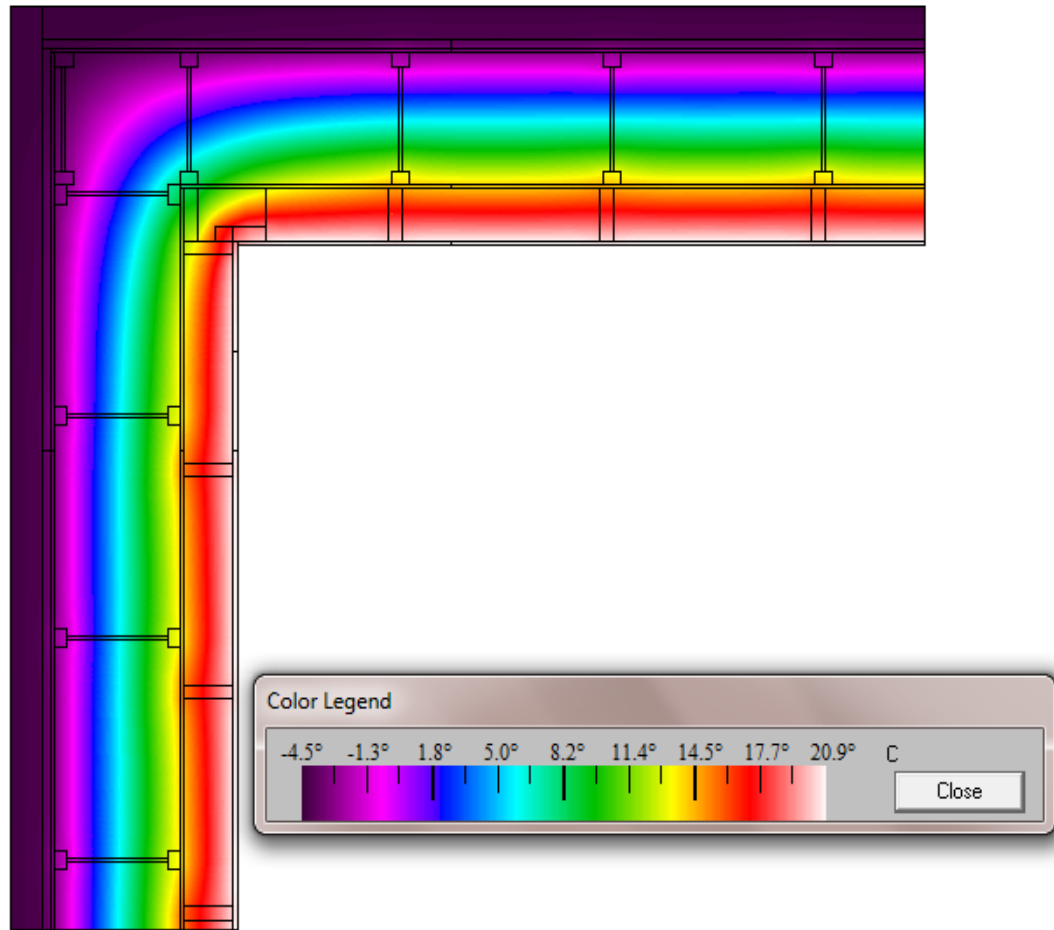
Figure N- 2: Passive House Outside Corner Ground Floor
