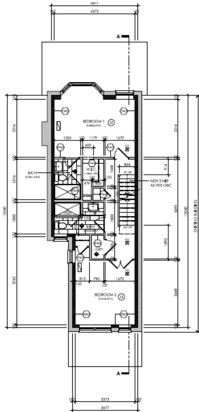
2 nd Floor
