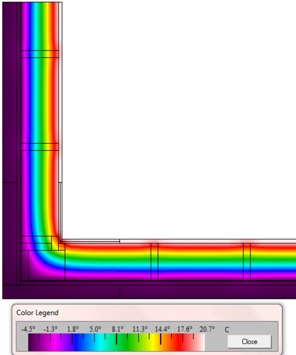
Figure L- 1: Typical Danish Outside Corner
