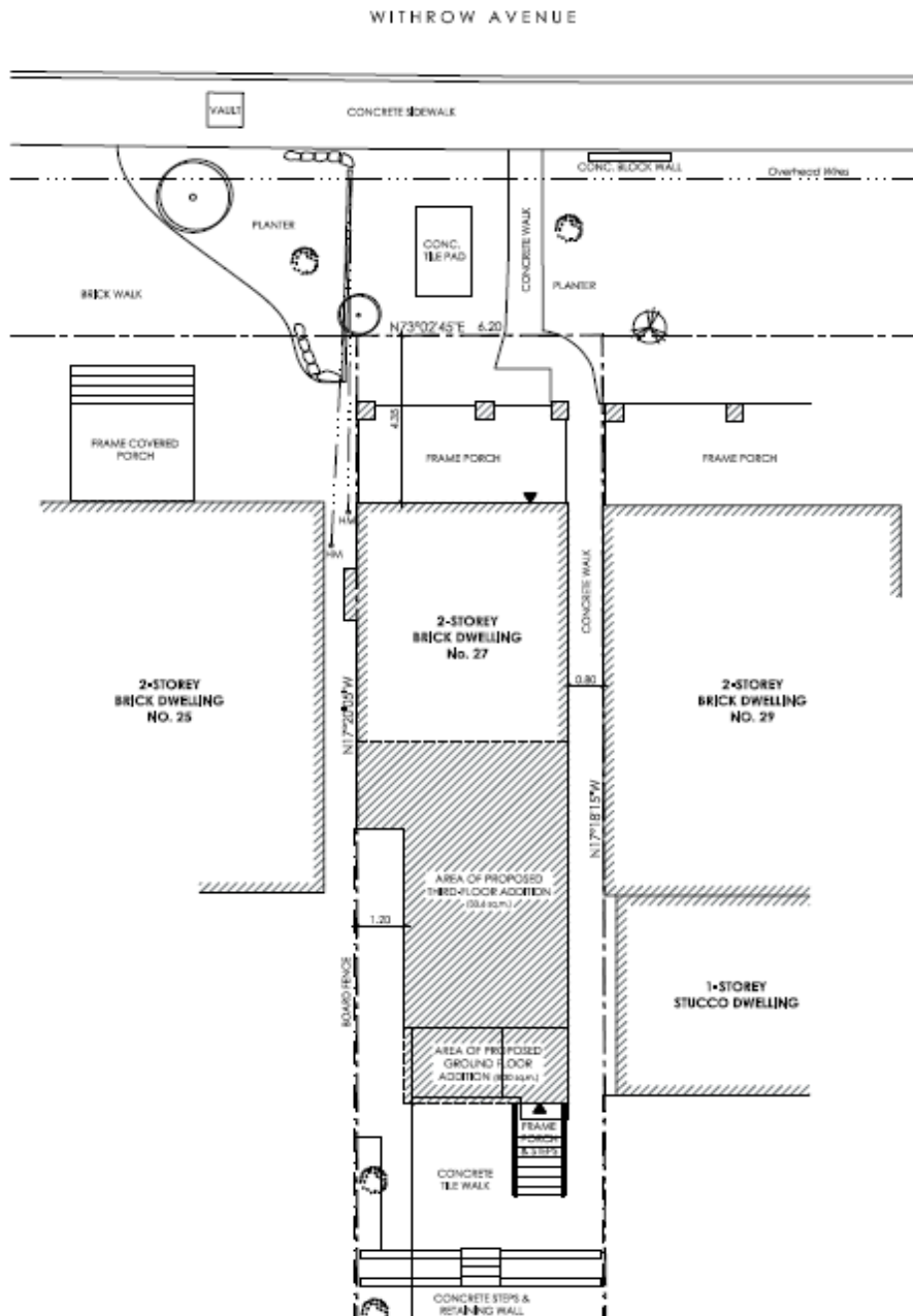
Site Plan
