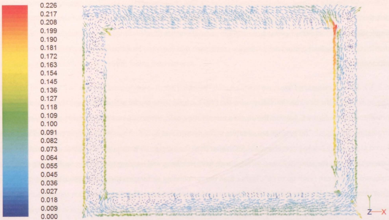
Figure 6.2 - Steady state basic geometry night time velocity (m/s) vectors ( y^+ = 46 )
