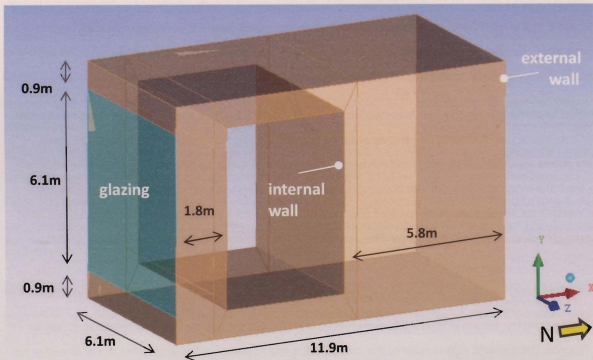
Figure 5.2 - 31 Sussex geometry
