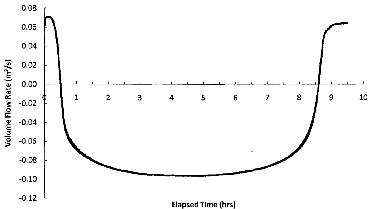
Figure 6.17 - Transient basic geometry volume flow rate
