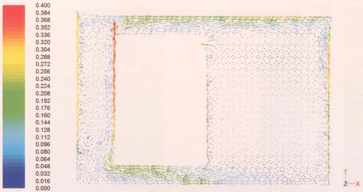
Figure 6.20 - Transient 3D Sussex geometry velocity (m/s) vectors, 12:00pm
