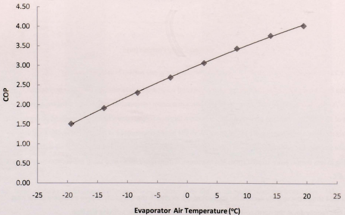
Figure 6.25 - Heat pump COP dependence on temperature
