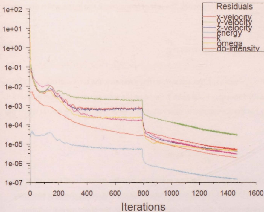
Figure 5.5 - Residual plot for basic geometry ( y^+ = 46 )
