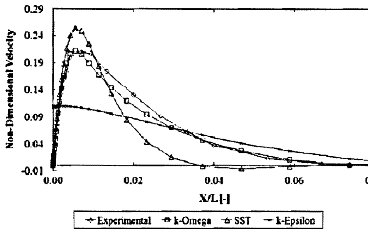
Figure 4.7 - Non-dimensional velocity profile from turbulence models and experiment (Rundle, 2011) Figure 4.8 - Atrium geometry (Rundle, 2011)
