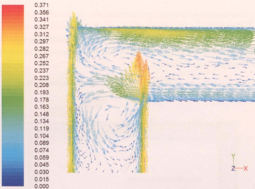
Figure 6.11 – Top left corner close-up of Figure 40 (m/s)
