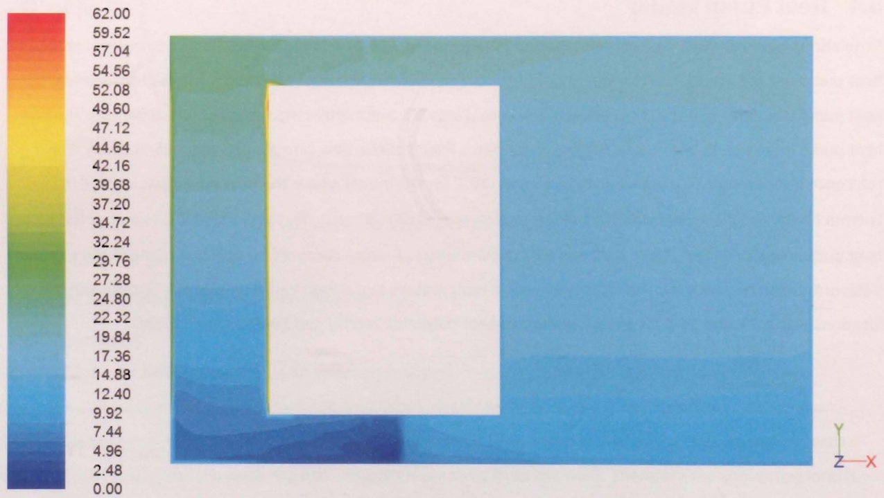
6.22 - Steady state 31 Sussex geometry temperature (°C) contours for heat pump model in bottom location ( y+ = 113 )
