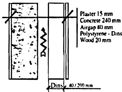
Figure 2.6 - Double-envelope wall construction
