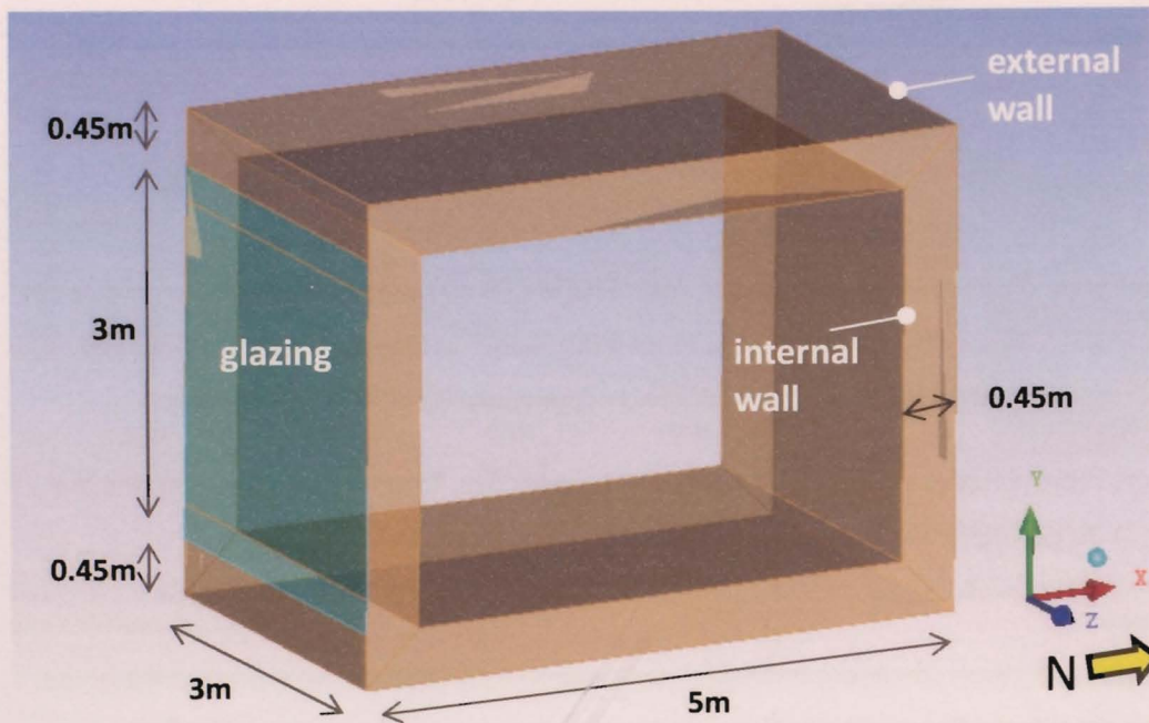
Figure 5.1 - Basic geometry
