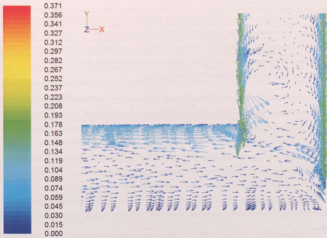
Figure 6.14 - Bottom right corner close-up of Figure 40 (m/s)
