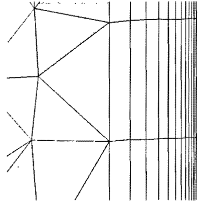
Figure 5.4 - Refined expanding mesh close-up
