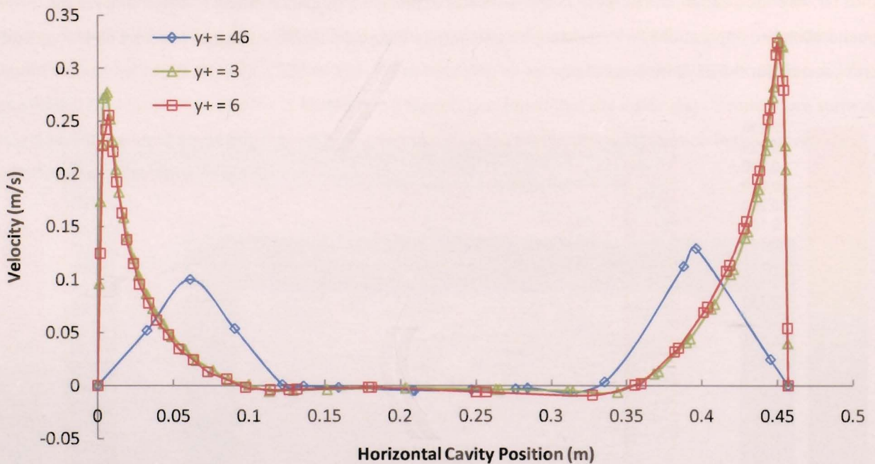
Figure 6.6 - Steady state Basic geometry horizontal velocity magnitude line plot for three mesh densities
