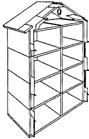
Figure 2.4 - Solar collector with double-envelope storage Figure 2.5 - Multi-storey double-envelope walls
