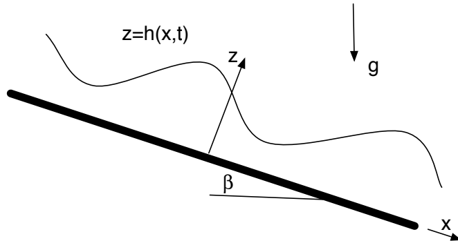
Figure 2.1: Schematic of the flow configuration.
