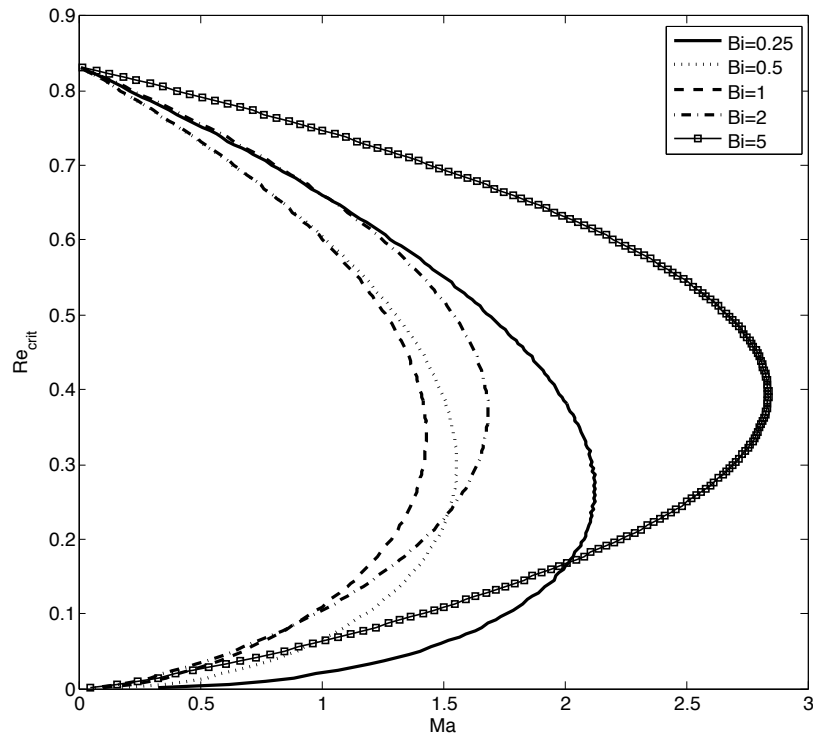
Figure 3.5: Re_{crit} as a function of Ma for \cot \beta = 1 , Pr = 7 , Ka = 100 , \alpha = 0 , \lambda = 0 and \Lambda = 0 .
