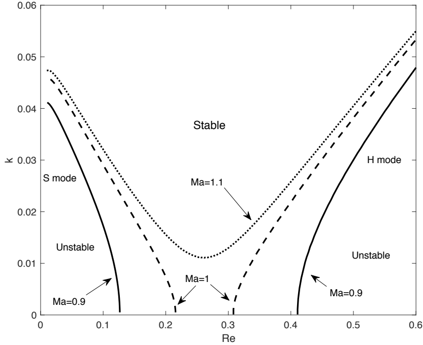
Figure 3.1: Neutral stability curves with \cot \beta = 1 , Pr = 7 , Ka = 100 , Bi = 1 , \alpha = 0.2 , \lambda = 0.2 and \Lambda = 0.2 .
