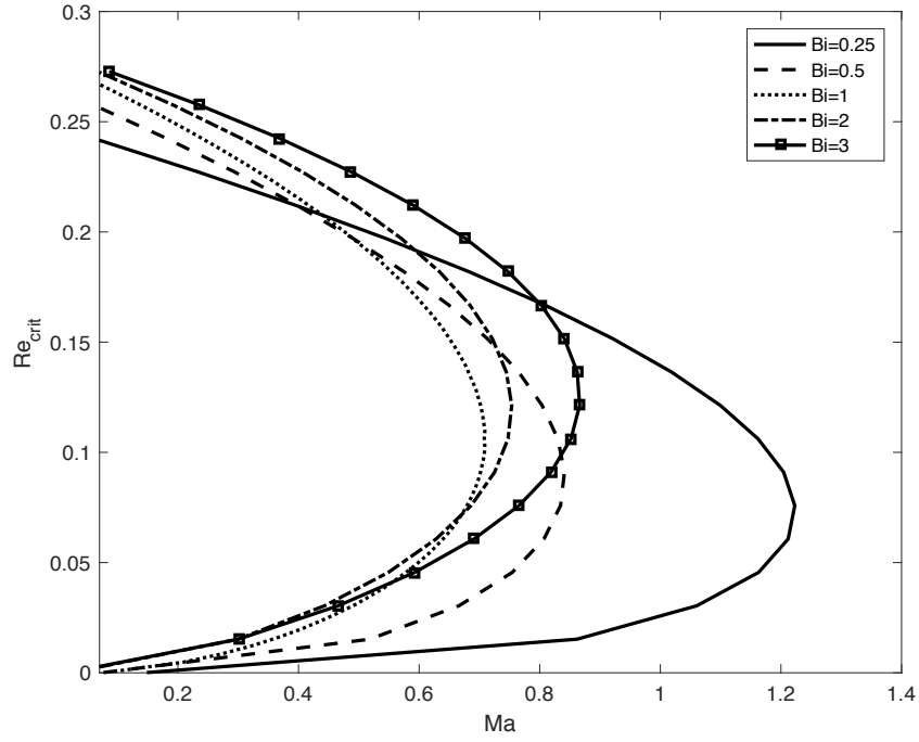
Figure 3.6: Re_{crit} as a function of Ma for \cot \beta = 1 , Pr = 7 , Ka = 100 , \alpha = 0 , \lambda = 0.5 and \Lambda = 0 .
