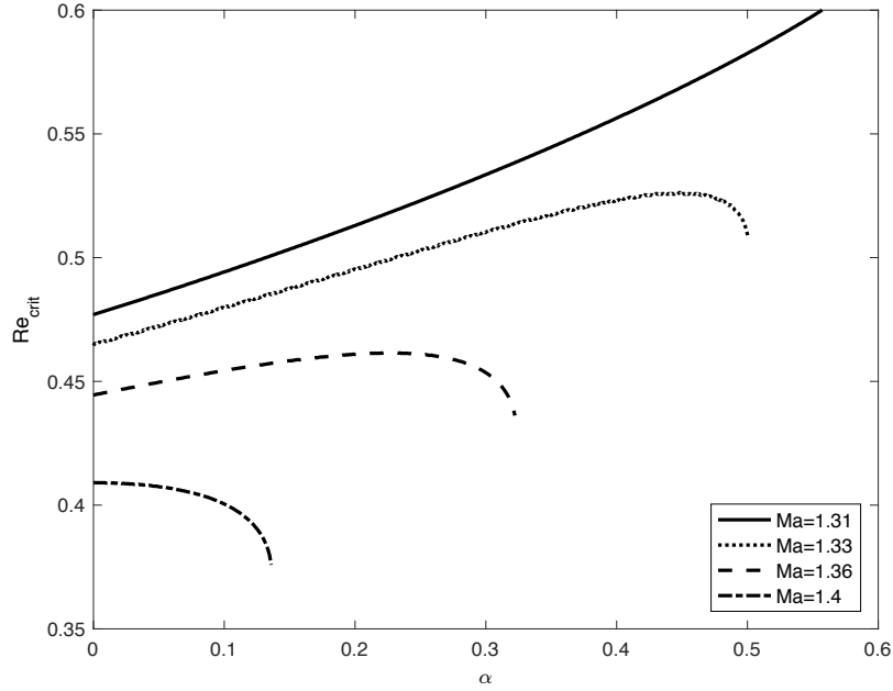
Figure 3.3: Re_{crit} for the H mode as a function of \alpha for \cot \beta = 1 , Pr = 7 , Ka = 100 , Bi = 1 , \lambda = 0 and \Lambda = 0 .
