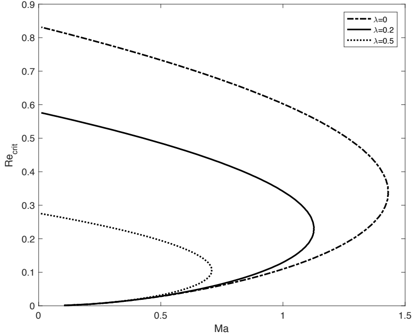
Figure 3.4: Re_{crit} as a function of Ma for \cot \beta = 1 , Pr = 7 , Ka = 100 , Bi = 1 , \alpha = 0 and \Lambda = 0 .
