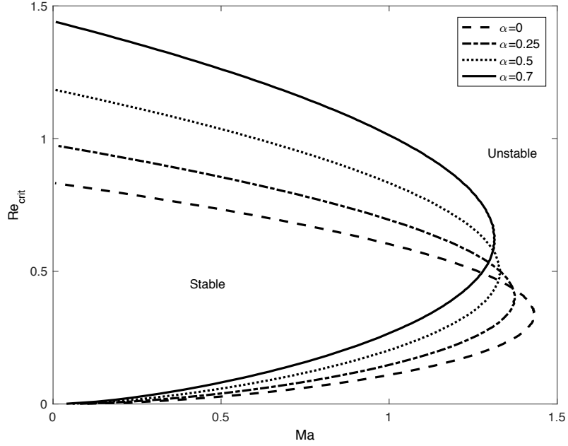
Figure 3.2: Re_{crit} as a function of Ma for \cot \beta = 1 , Pr = 7 , Ka = 100 , Bi = 1 , \lambda = 0 and \Lambda = 0 .
