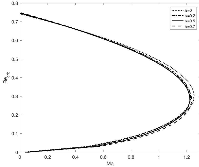
Figure 3.7: Re_{crit} as a function of Ma for \cot \beta = 1 , Pr = 7 , Ka = 100 , Bi = 1 , \alpha = 0.1 and \lambda = 0.2 .
